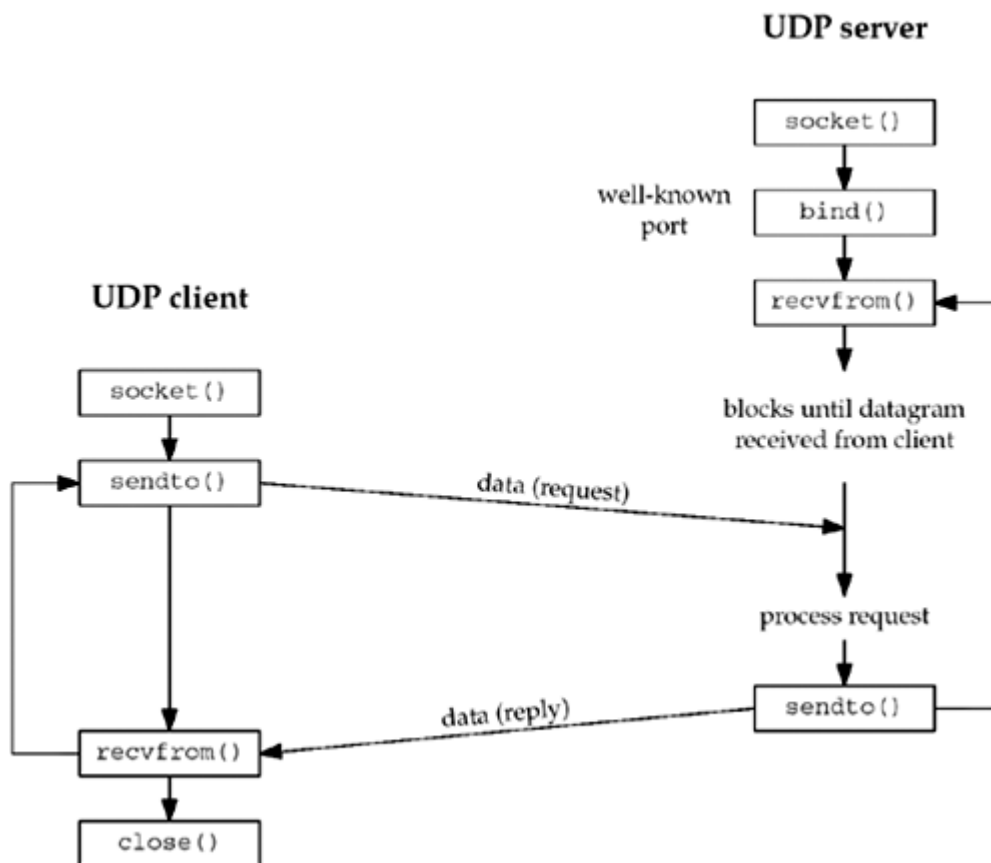
Figure 8.1. Socket functions for UDP client/server.
