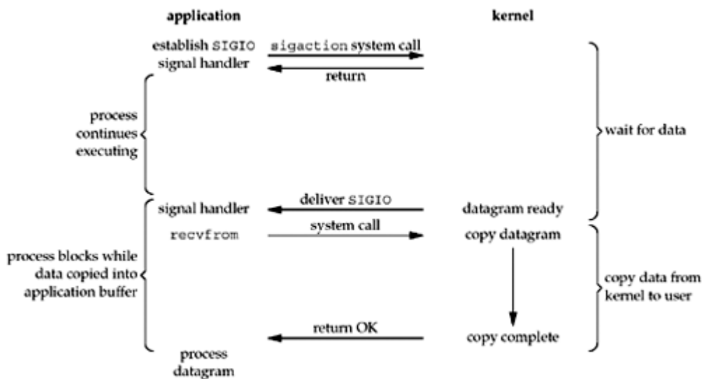
Figure 6.4. Signal-Driven I/O model.
