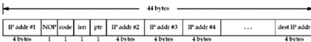
Figure 27.4. Format of source route option returned by getsockopt .
