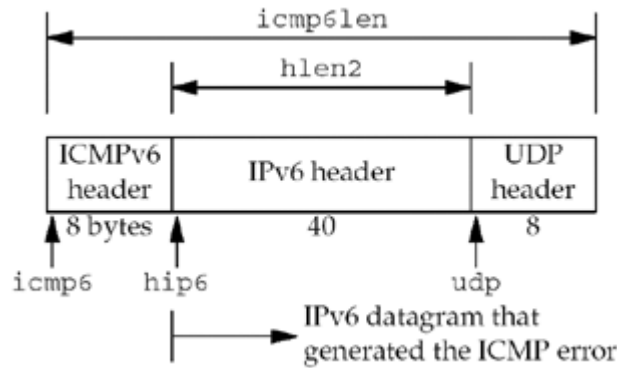
Figure 28.22. Headers, pointers, and lengths in processing ICMPv6 error.
