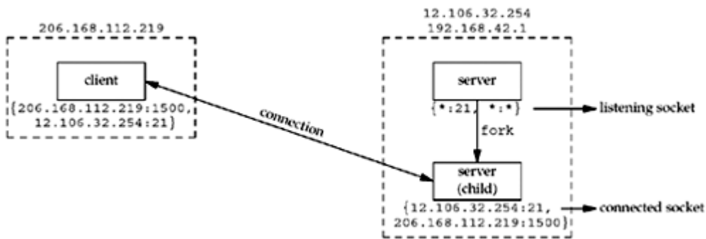
Figure 2.13. Concurrent server has child handle client.
