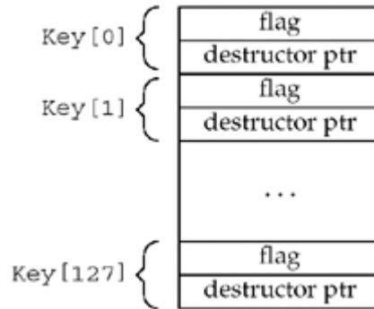
Figure 26.7. Possible implementation of thread-specific data.
