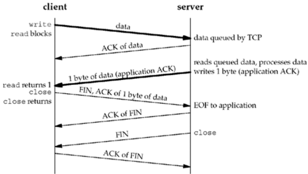
Figure 7.11. Application ACK.
