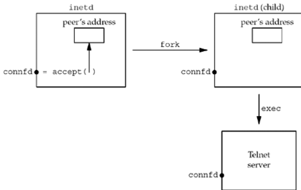
Figure 4.18. Example of inetd spawning a server.
