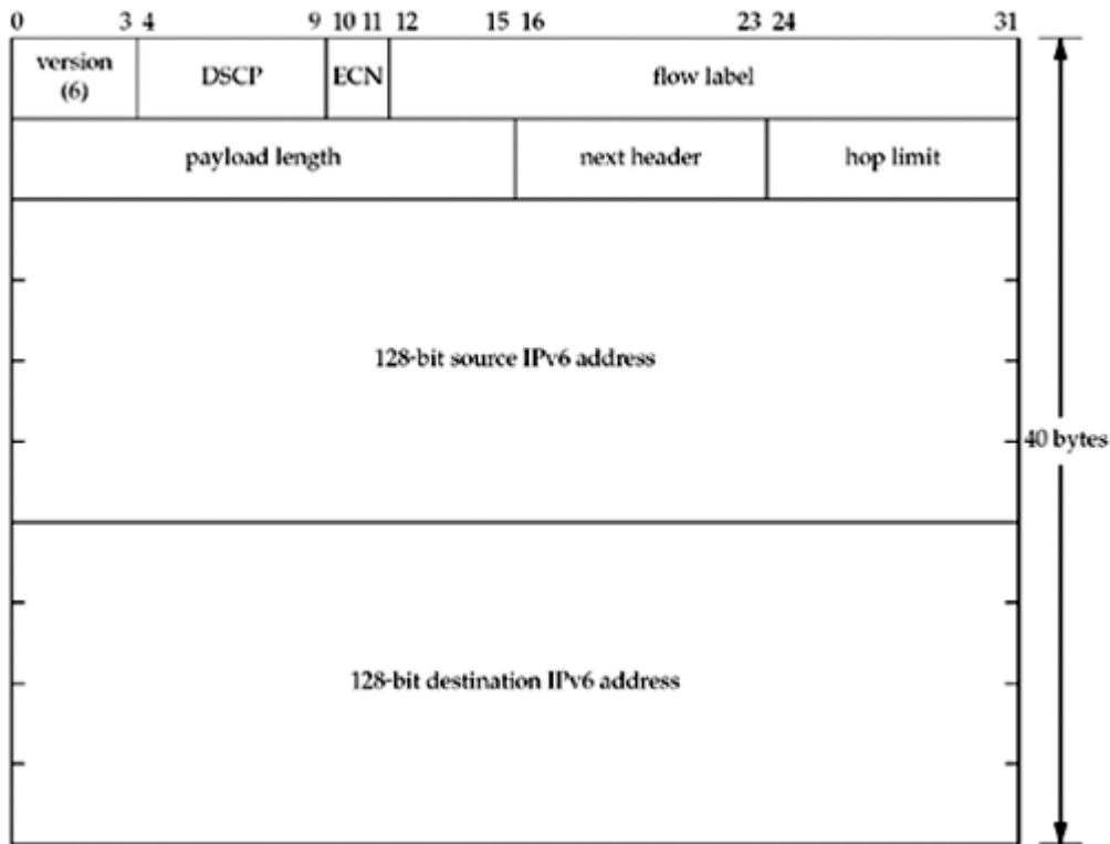
Figure A.2. Format of the IPv6 header.
