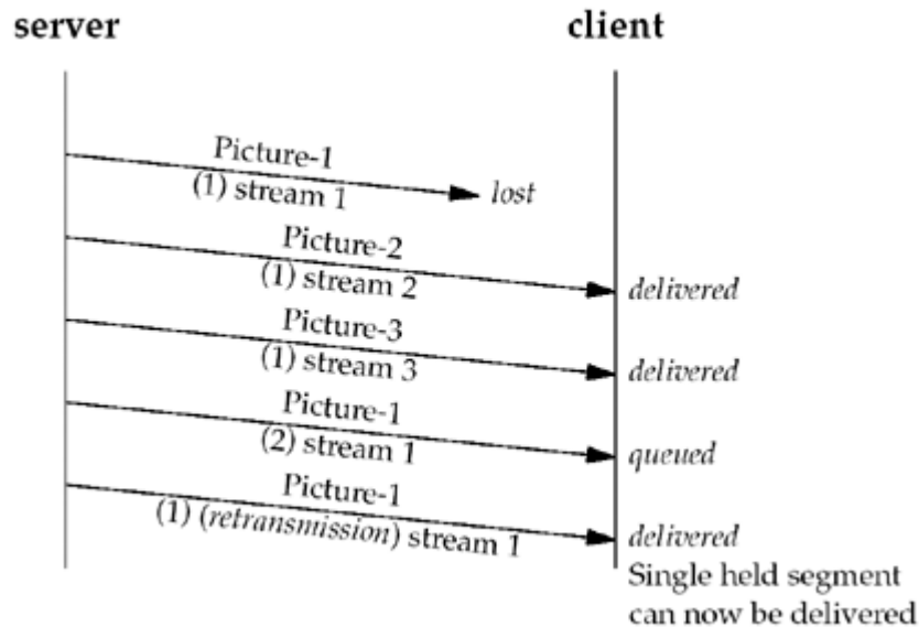
Figure 10.6. Sending three pictures over three SCTP streams.
