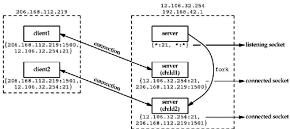
Figure 2.14. Second client connection with same server.
