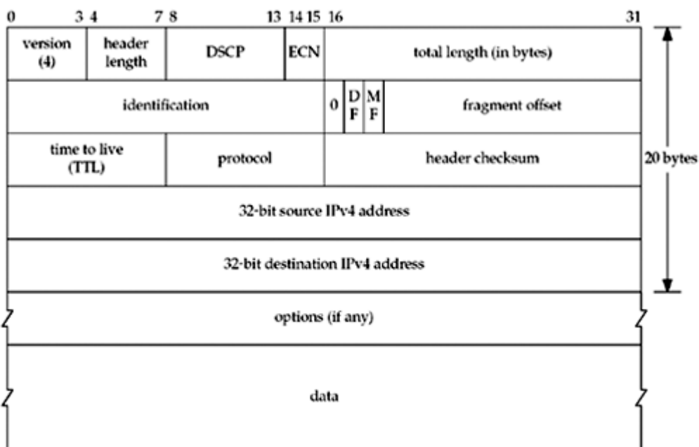
Figure A.1. Format of the IPv4 header.
