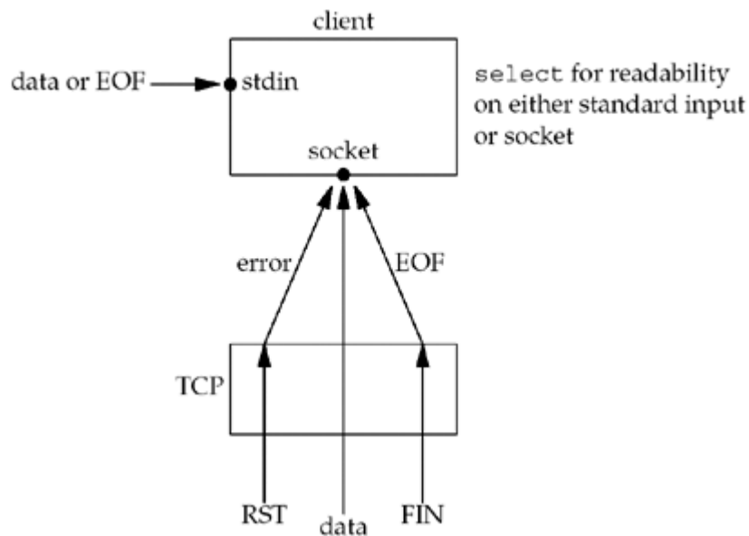
Figure 6.8. Conditions handled by select in str_cli .
