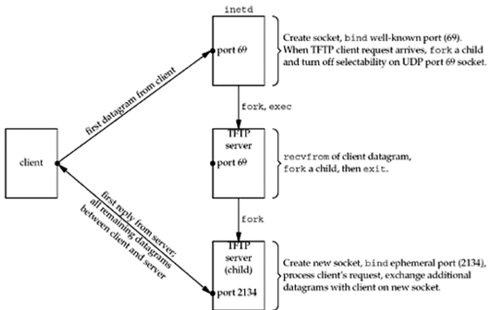
Figure 22.20. UDP concurrent server invoked by inetd .
