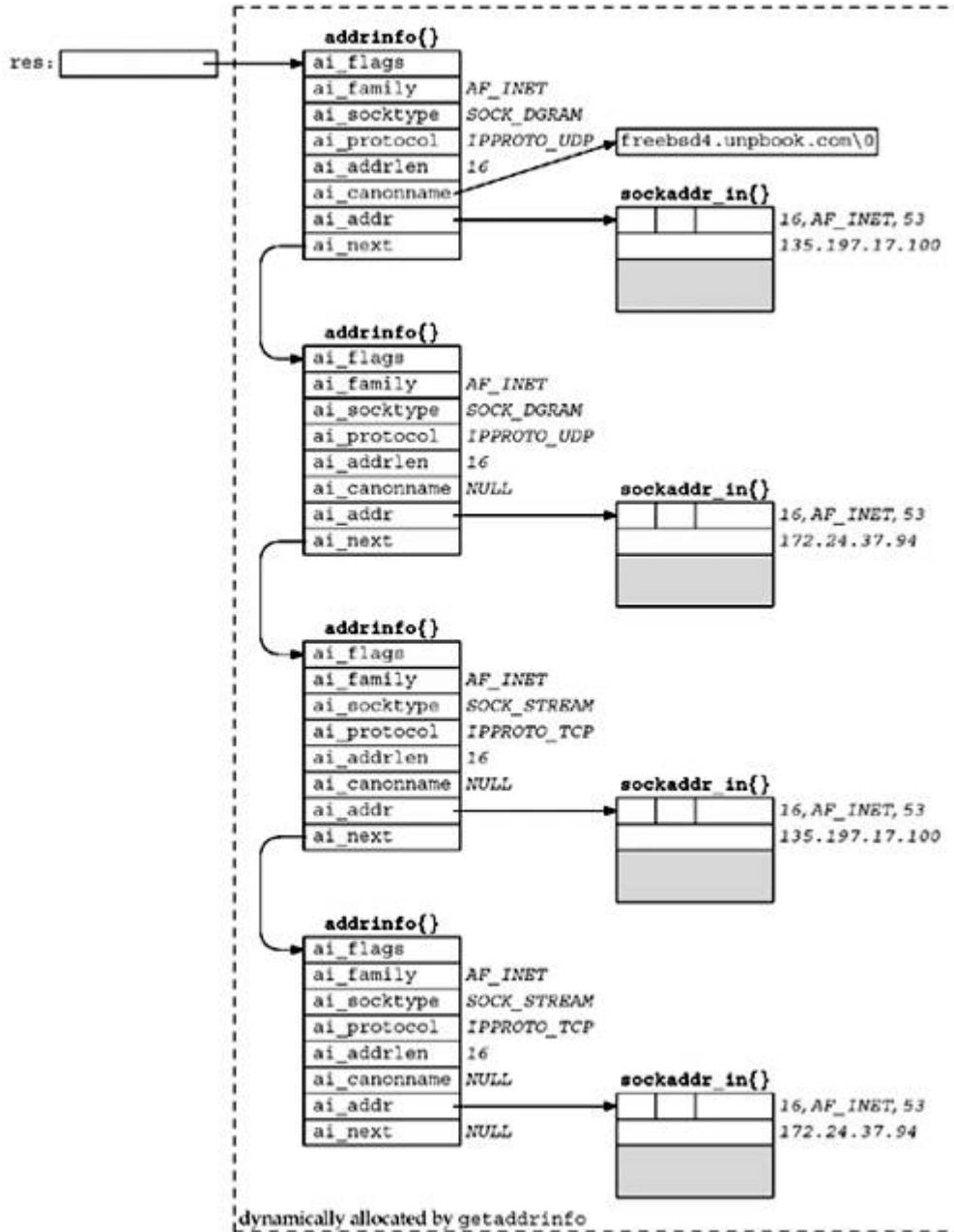
Figure 11.5. Example of information returned by getaddrinfo .
