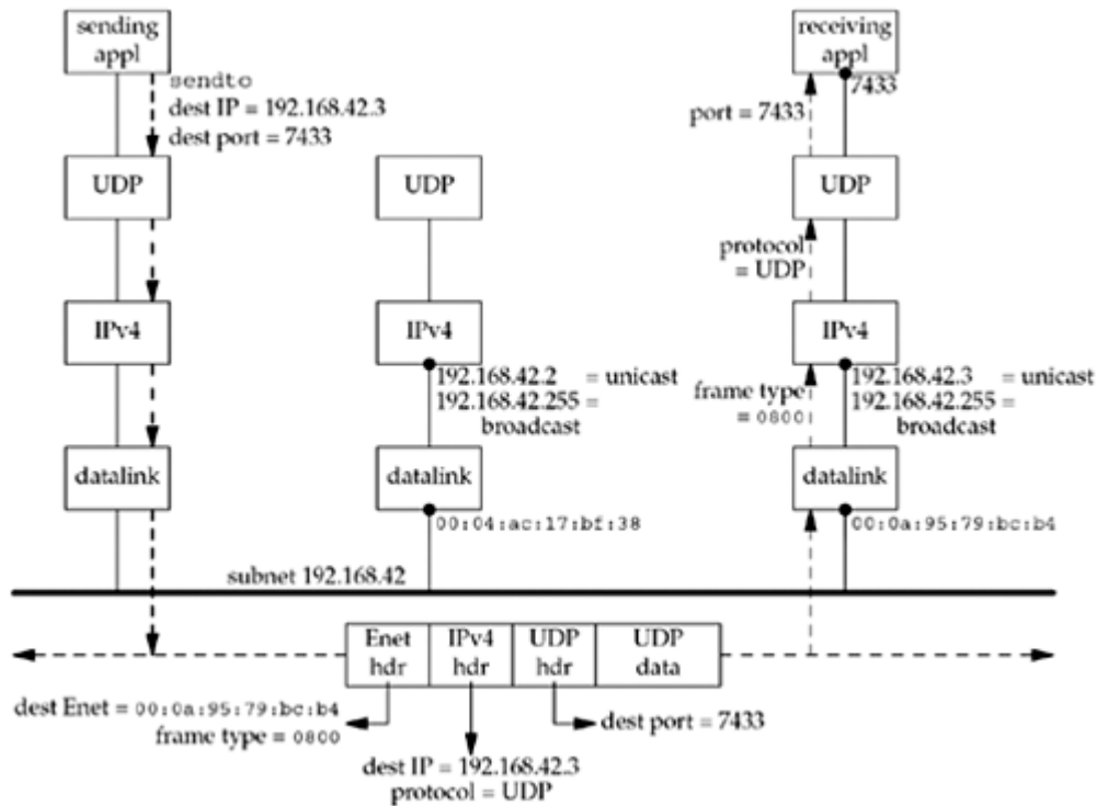
Figure 20.3. Unicast example of a UDP datagram.
