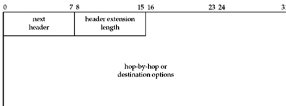
Figure 27.7. Format of hop-by-hop and destination options.
