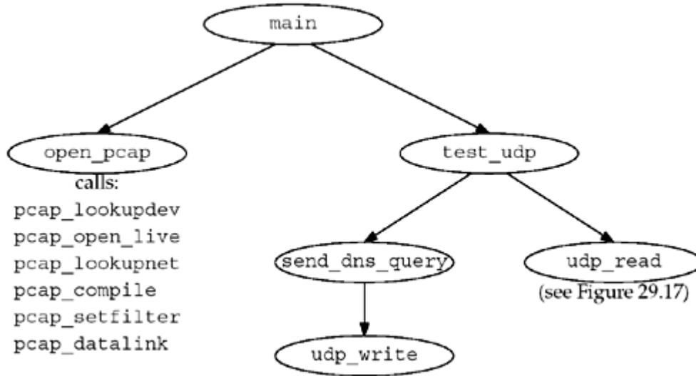
Figure 29.4. Summary of functions for our udpcksum program.
