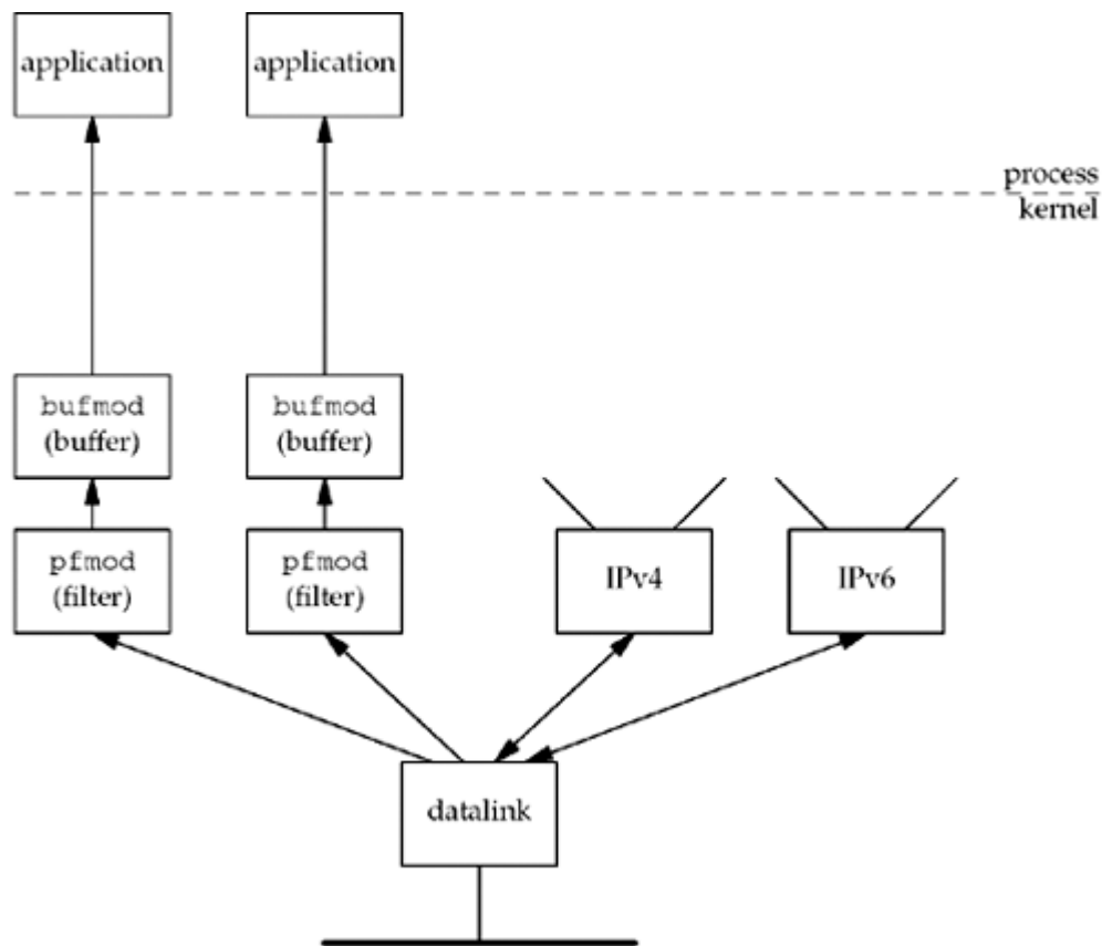
Figure 29.2. Packet capture using DLPI, pfmod , and bufmod .
