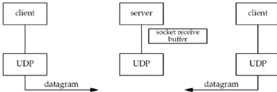
Figure 8.6. Summary of UDP client/server with two clients.
