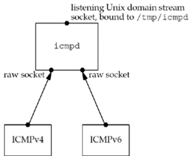
Figure 28.26. icmpd daemon: initial sockets created.
