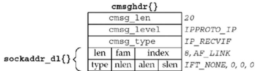
Figure 22.3. Ancillary data object returned for IP_RECVIF .
