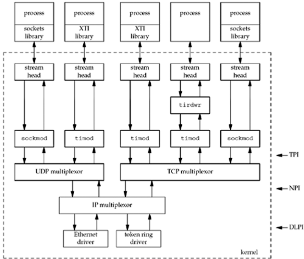
Figure 31.3. A potential implementation of TCP/IP using STREAMS.
