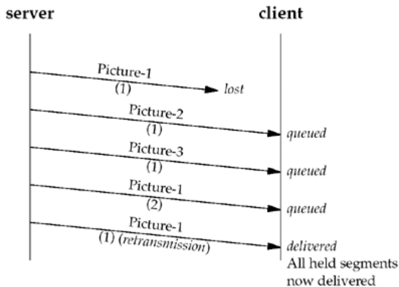
Figure 10.5. Sending three pictures over one TCP connection.
