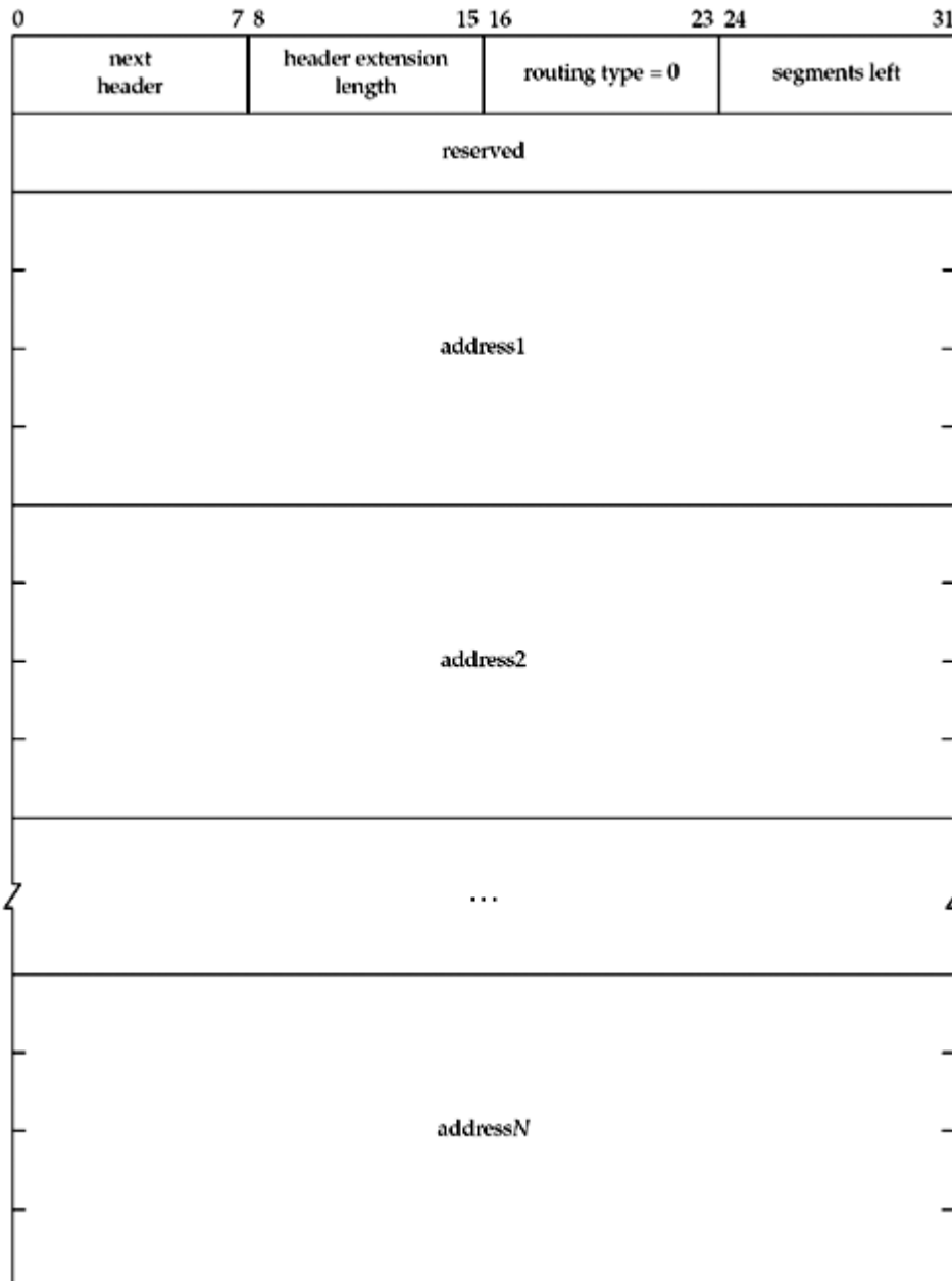
Figure 27.11. IPv6 routing header.
