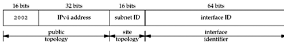
Figure B.3. 6to4 addresses.
