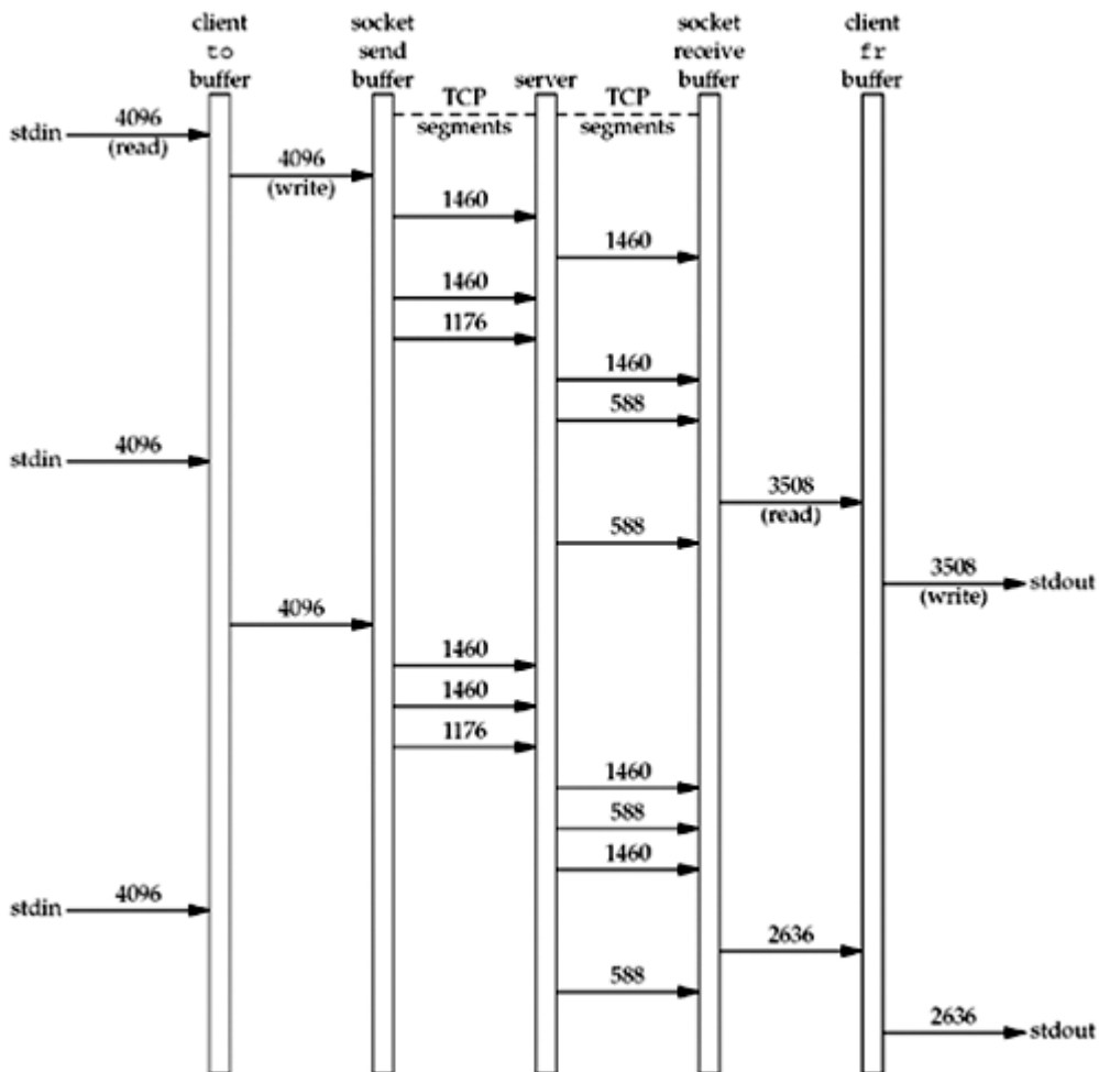
Figure 16.8. Timeline of nonblocking example.
