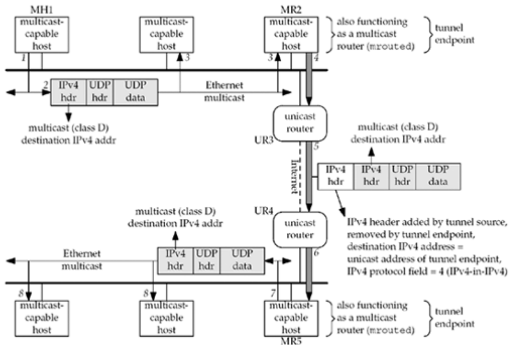
Figure B.1. IPv4-in-IPv4 encapsulation used on MBone.
