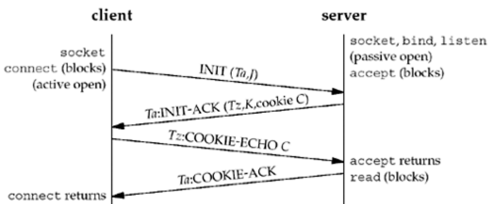
Figure 2.6. SCTP four-way handshake.
