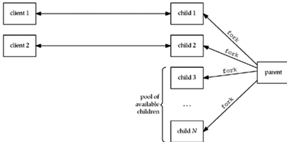
Figure 30.8. Preforking of children by server.
