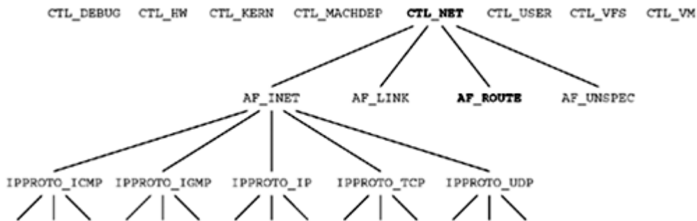
Figure 18.11. Hierarchical arrangement of sysctl names.
