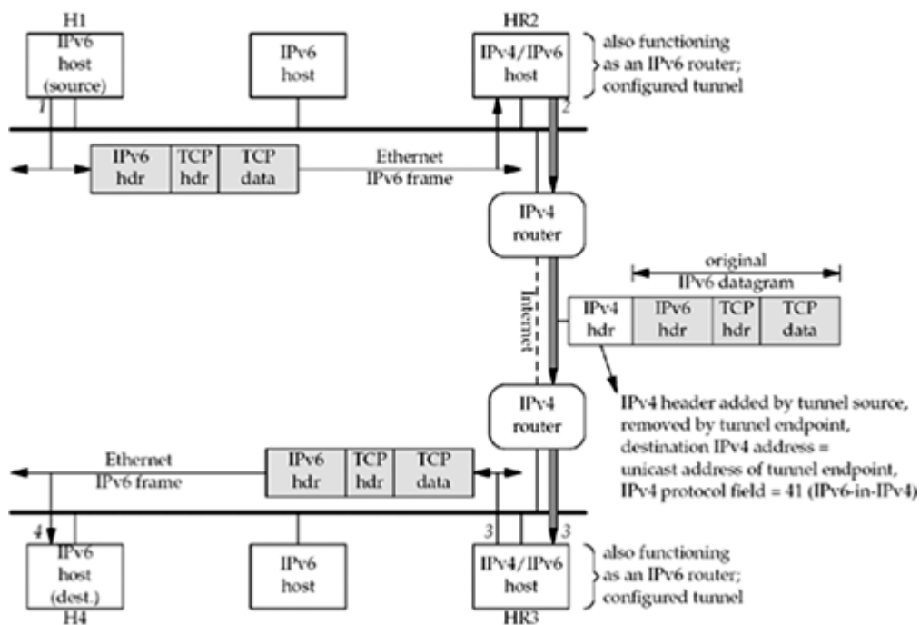
Figure B.2. IPv6-in-IPv4 encapsulation on 6bone.
