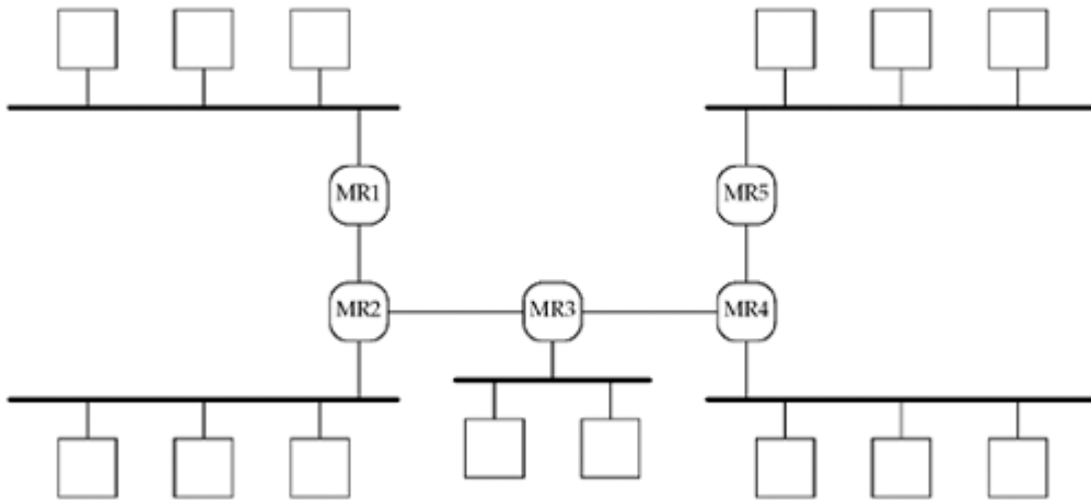
Figure 21.5. Five LANs connected with five multicast routers.
