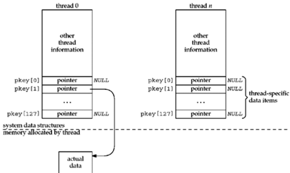
Figure 26.9. Associating malloced region with thread-specific data pointer.
