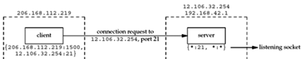
Figure 2.12. Connection request from client to server.
