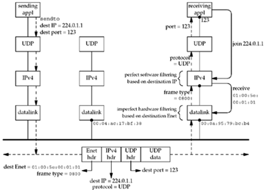
Figure 21.4. Multicast example of a UDP datagram.
