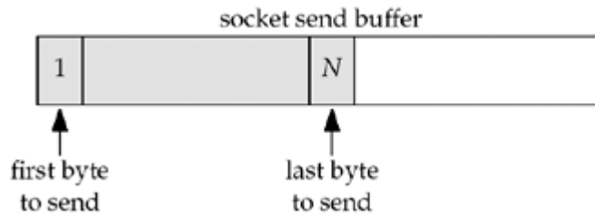
Figure 24.1. Socket send buffer containing data to send.
