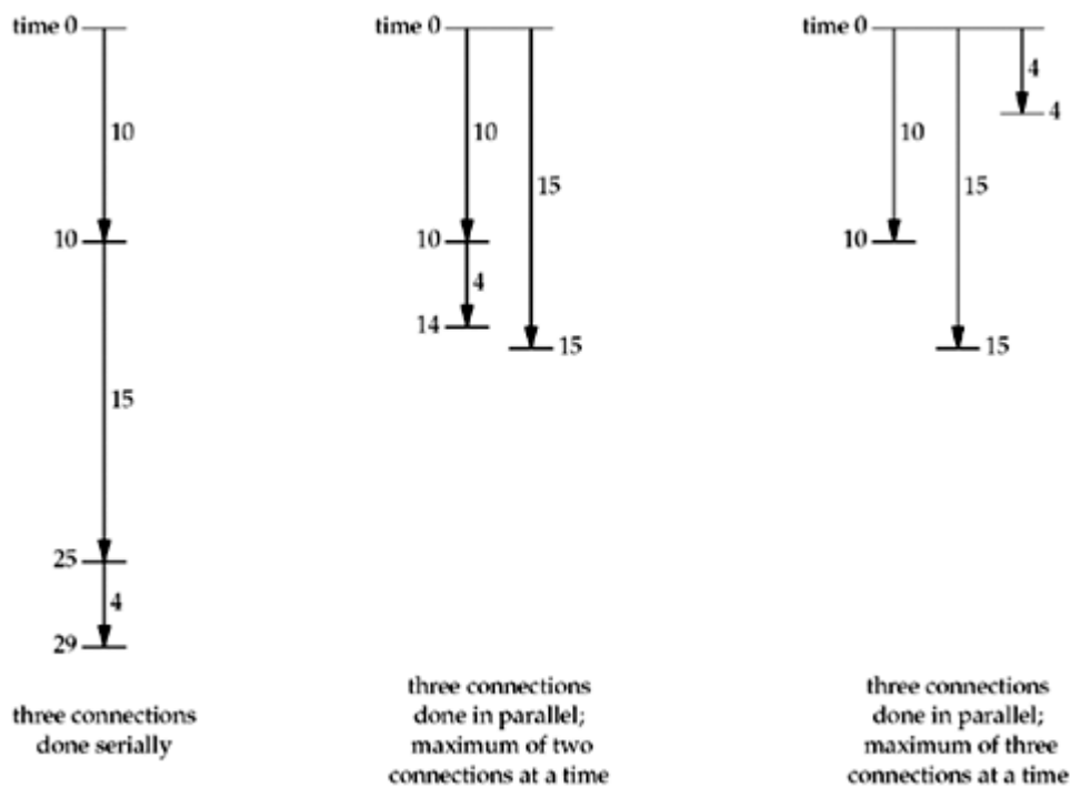
Figure 16.12. Establishing multiple connections in parallel.
