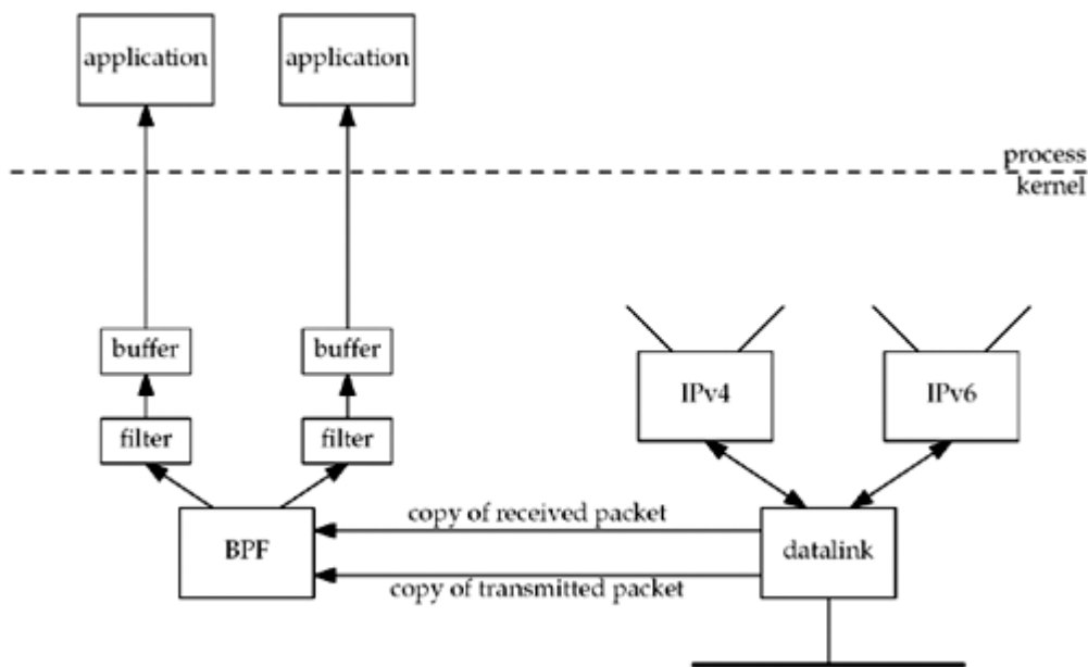
Figure 29.1. Packet capture using BPF.
