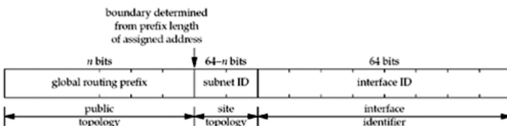
Figure A.8. IPv6 aggregatable global unicast addresses.
