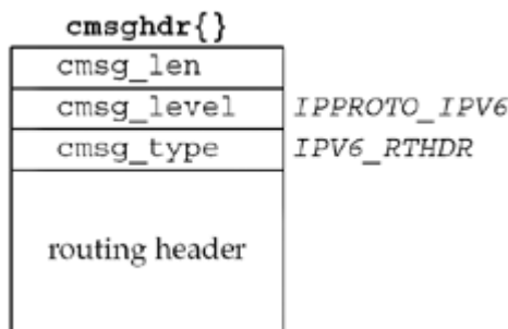
Figure 27.12. Ancillary data object for IPv6 routing header.
