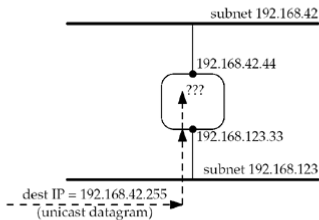
Figure 20.2. Does a router forward a subnet-directed broadcast?
