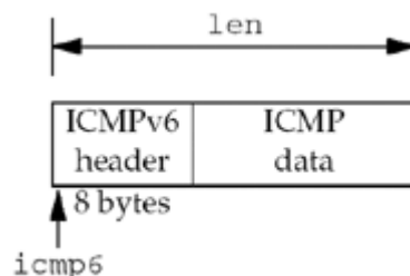
Figure 28.11. Headers, pointers, and lengths in processing ICMPv6 reply.
