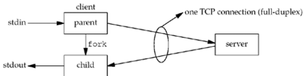
Figure 16.9. str_cli function using two processes.
