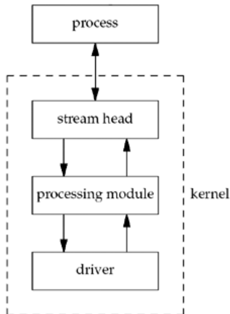
Figure 31.2. A stream with a processing module.
