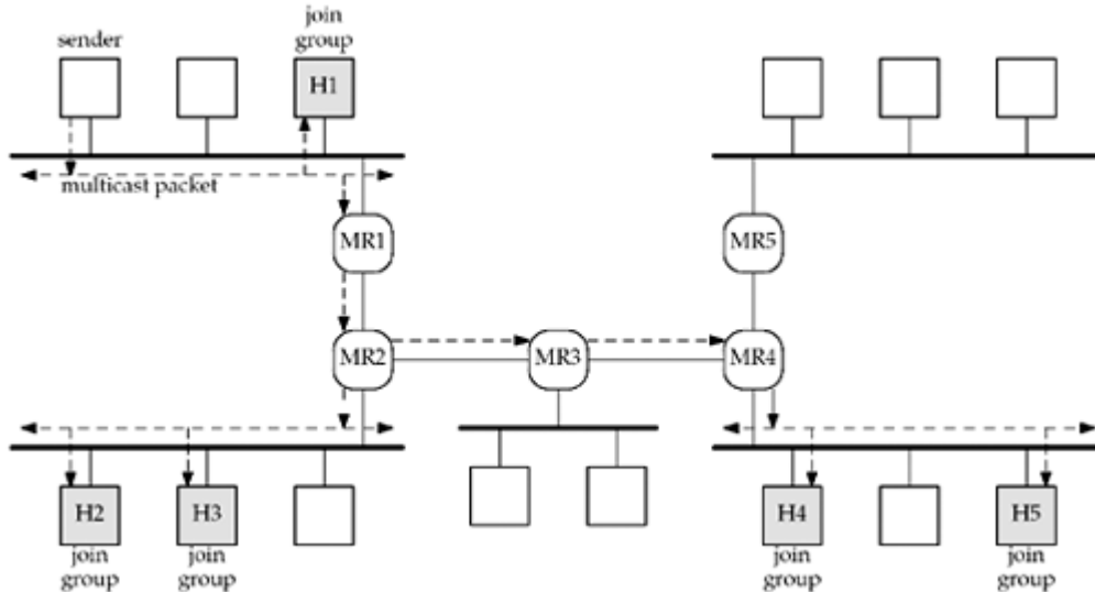
Figure 21.7. Sending multicast packets on a WAN.
