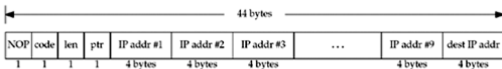
Figure 27.1. Passing a source route to the kernel.
