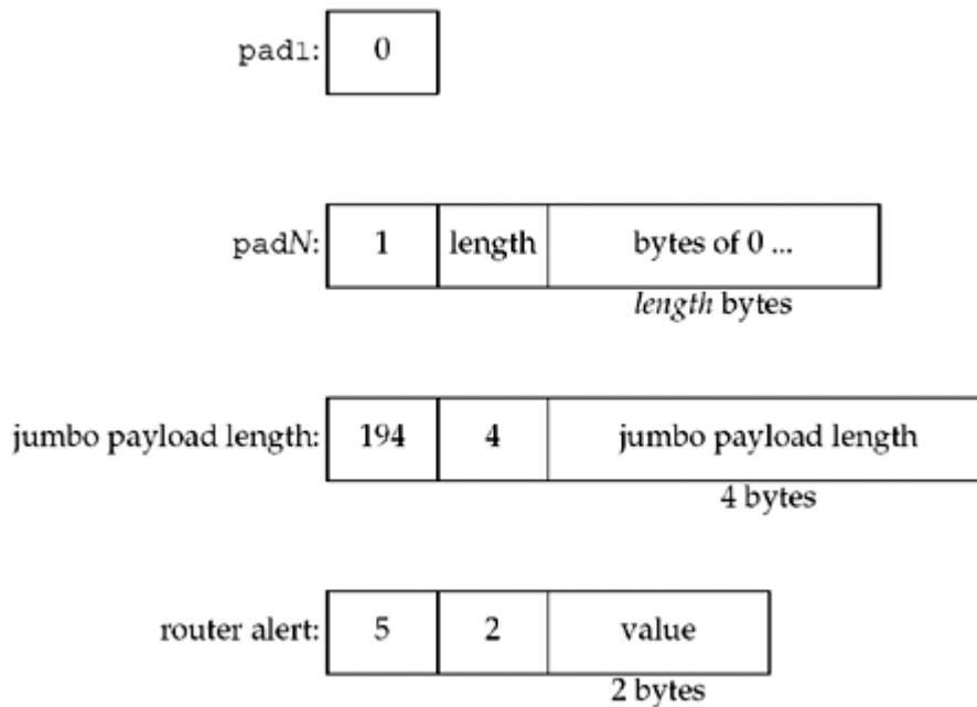
Figure 27.9. IPv6 hop-by-hop options.
