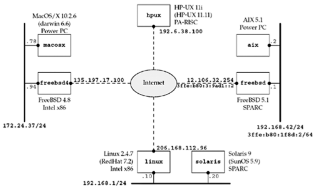
Figure 1.16. Networks and hosts used for most examples in the text.
