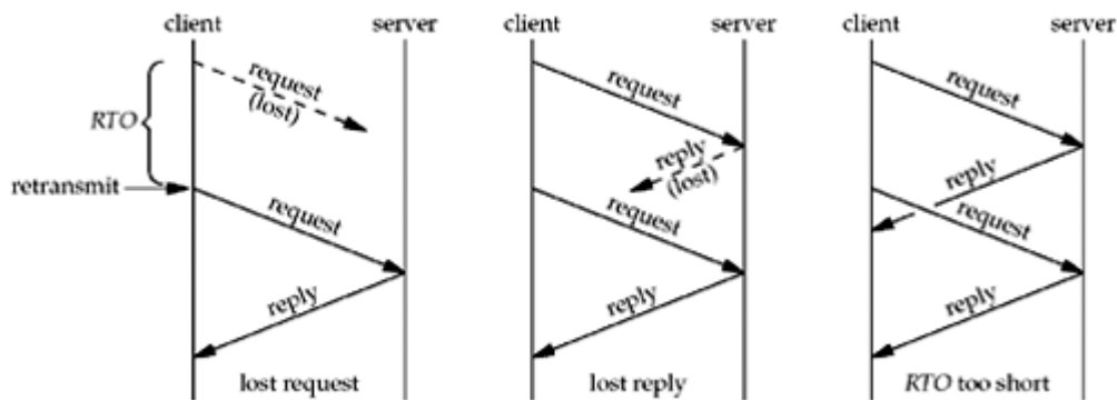
Figure 22.5. Three scenarios when retransmission timer expires.
