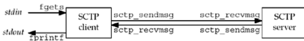
Figure 10.1. Simple SCTP streaming echo client and server.
