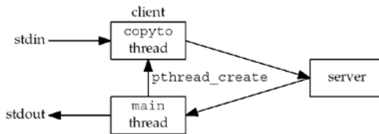
Figure 26.1. Recoding str_cli to use threads.
