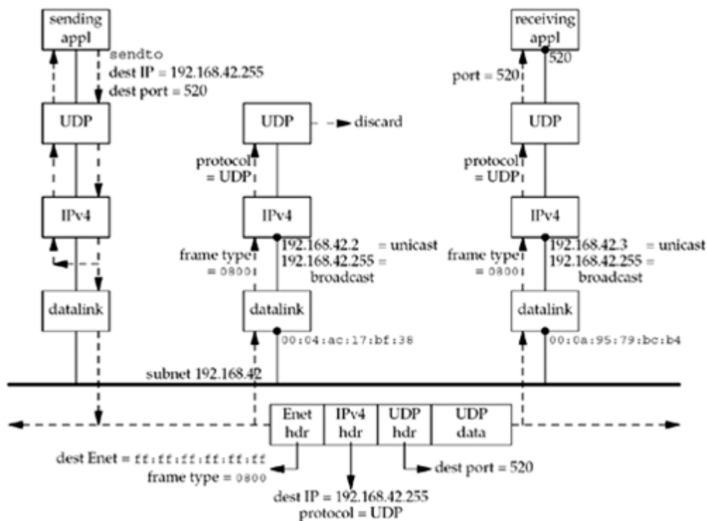
Figure 20.4. Example of a broadcast UDP datagram.
